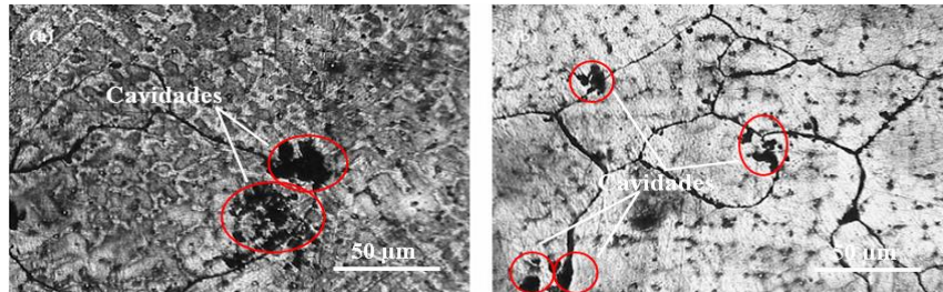
Figure 4(a) and (b). Blade surface cavities for 27 % concentration.
