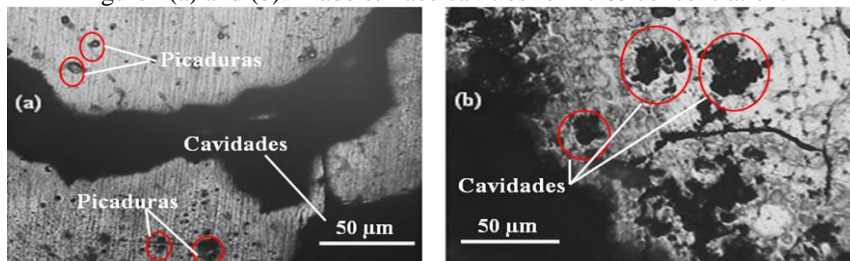
Figure 5(a) and (b). Blade surface cavities for 34% concentrations.
