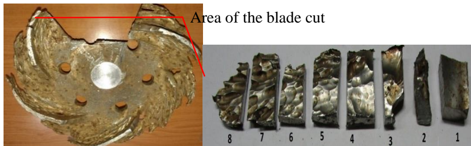
Figure 1. Cut made to a blade of selected samples.
